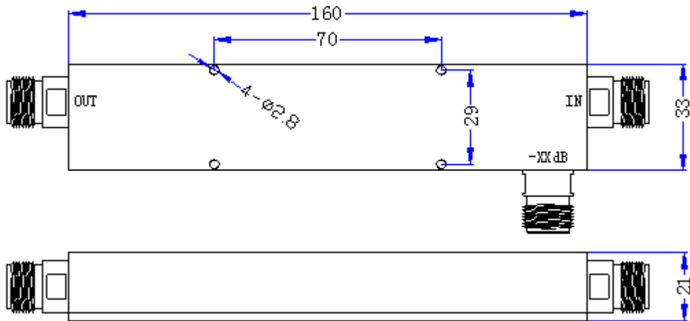
Figure 1 JX-DC-340M2000M-6/10/15/20/30N front panel layout
